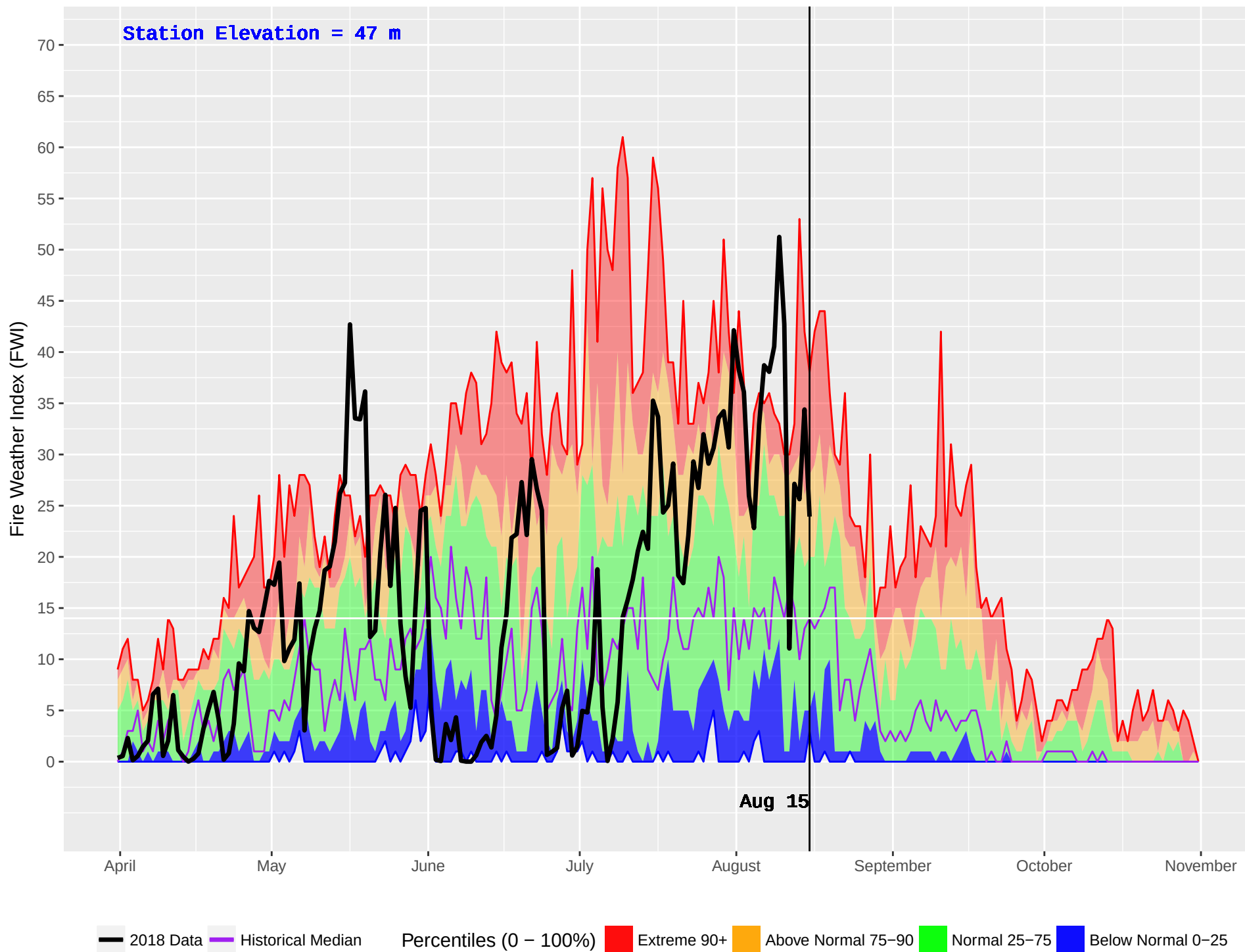
HAGENSBORG 2 (904) : Historical (2005–2016) and Current (2018) Daily Fire Weather Index (FWI)
